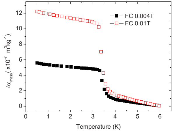
FIG. 3. (Color online) Temperature dependence of magnetic susceptibility of \text{LaCoO}_{2.98\pm 0.02} cooled in a field of 4 and 10 mT and measured in a residual field of 10 \mu\text{T} .
