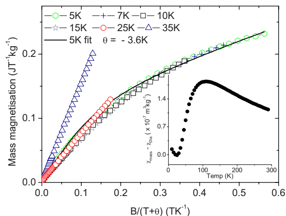
FIG. 1. (Color online) Mass magnetization curves for LaCoO 2.98 as a function of temperature up to 5 T, demonstrating scaling behavior from 5–25 K. Details of the fit to the 5 K data (solid line) are described in the text. The inset shows the temperature dependence of the susceptibility measured in 5 T.
