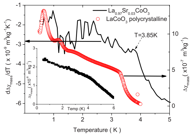
FIG. 4. (Color online) Temperature dependence of magnetic susceptibility of the polycrystalline \text{LaCoO}_{2.96\pm 0.02} (circles) and the derivative of the susceptibility of \text{La}_{0.97}\text{Sr}_{0.03}\text{CoO}_3 (line). Both samples were cooled in a field of 10 mT and measured in a residual field of 10 \mu\text{T} . The inset shows the temperature dependence of the susceptibility for \text{La}_{0.97}\text{Sr}_{0.03}\text{CoO}_3 .
