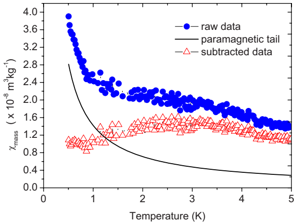
FIG. 2. (Color online) Temperature dependence of magnetic susceptibility of \text{LaCoO}_{2.98\pm 0.02} cooled and measured in a residual field of 10 \mu\text{T} . The raw data along with the subtraction of the paramagnetic fit are shown.
